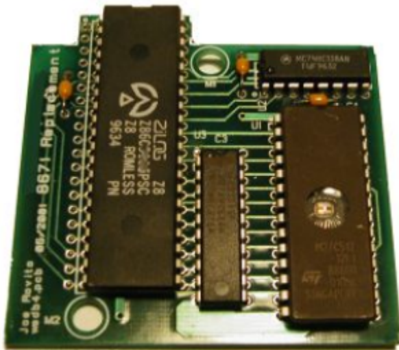
Z8671 Replacement Board, Joe Rovito, circa 2001, Bild von http://www.ntrd.com/joe/z8671.htm
